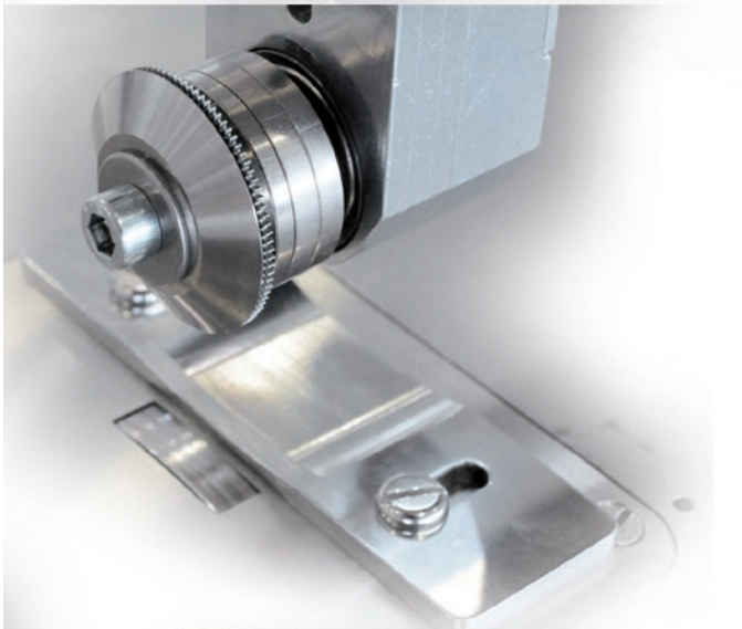
Extra-small anvil wheel to weld narrow radii and tight curves (e.g. welding bras or medical items)
